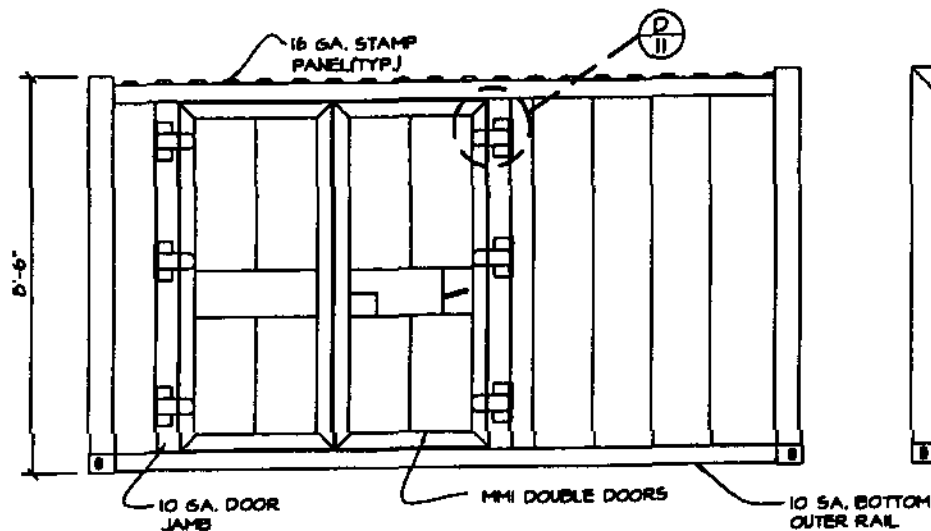
EXTERIOR ELEVATION C
