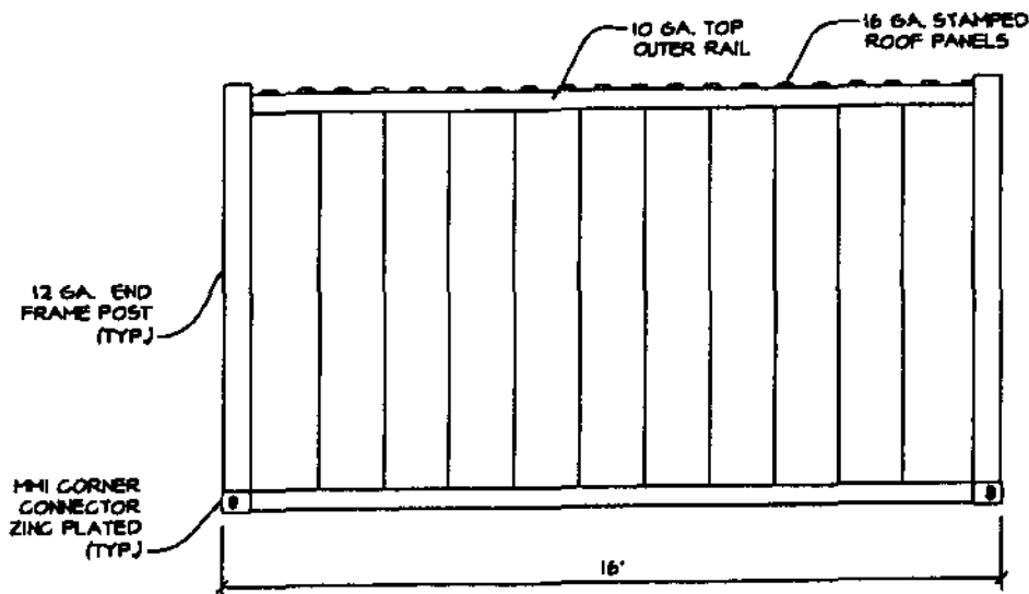
EXTERIOR ELEVATION A
