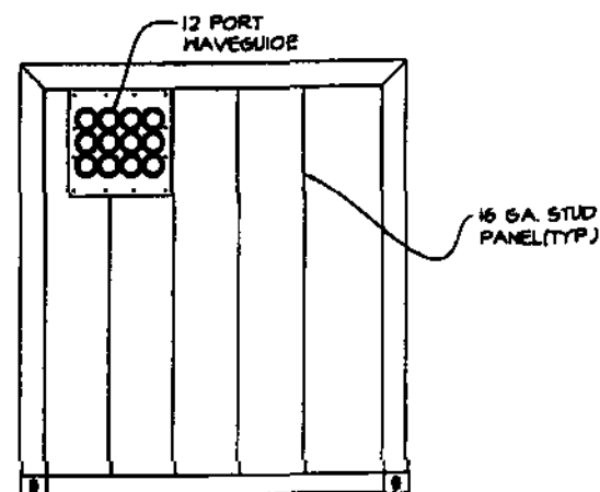
EXTERIOR ELEVATION B
